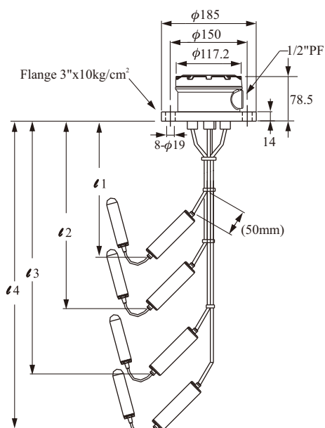
MODEL: FBX10000-□□□□□C
