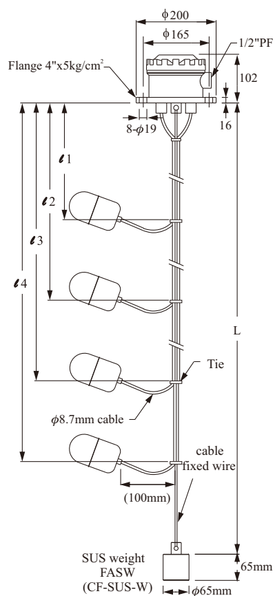
MODEL: FBX10000-□□□□□B
