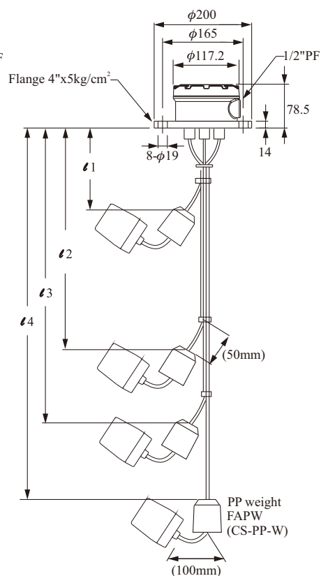
MODEL: FBX10000-□□□□□C
