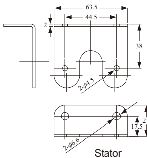
Stator
